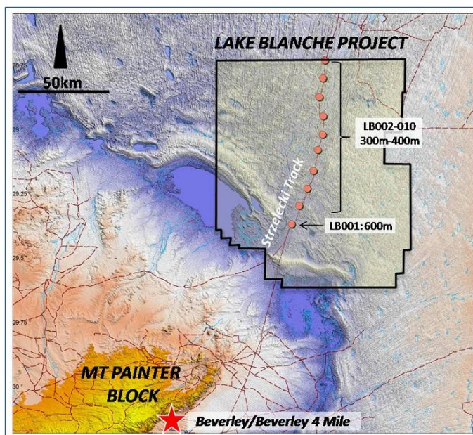
Figure 2: Drillhole locations superimposed on digital elevation model: Lake Blanche area
