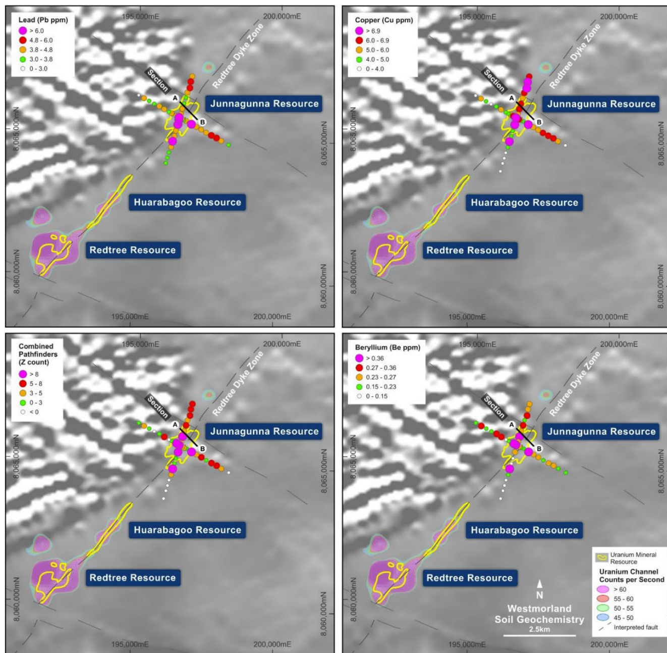
Figure 6: Orientation soil geochemistry carried out by DevEx in collaboration with Laramide at the Junnagunna uranium deposit. Pathfinder geochemistry successfully pin-points the underlying uranium mineralisation. Junnagunna forms part of the larger Westmoreland Uranium mineral resource estimate, but is masked by surficial regolith and displays no surface uranium signature in both soils and radiometric surveys.
